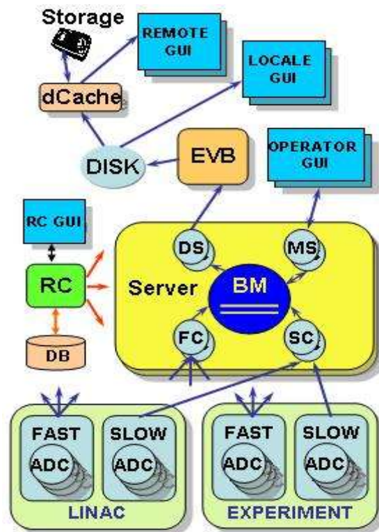
Figure 1: DAQ layout
