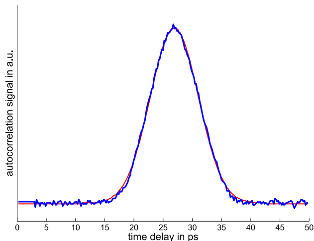
Figure 3: Auto correlating function of laser pulses (blue) and Gaussian fit (red) FWHM width of 10.16 ps.
