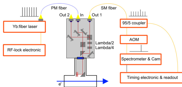
Figure 1: Experimental setup.
