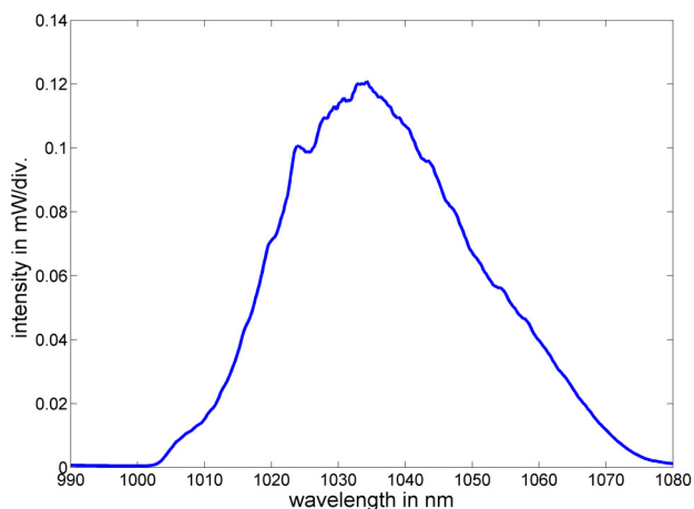
Figure 4: Optical spectrum of pre-amplified laser pulses.
