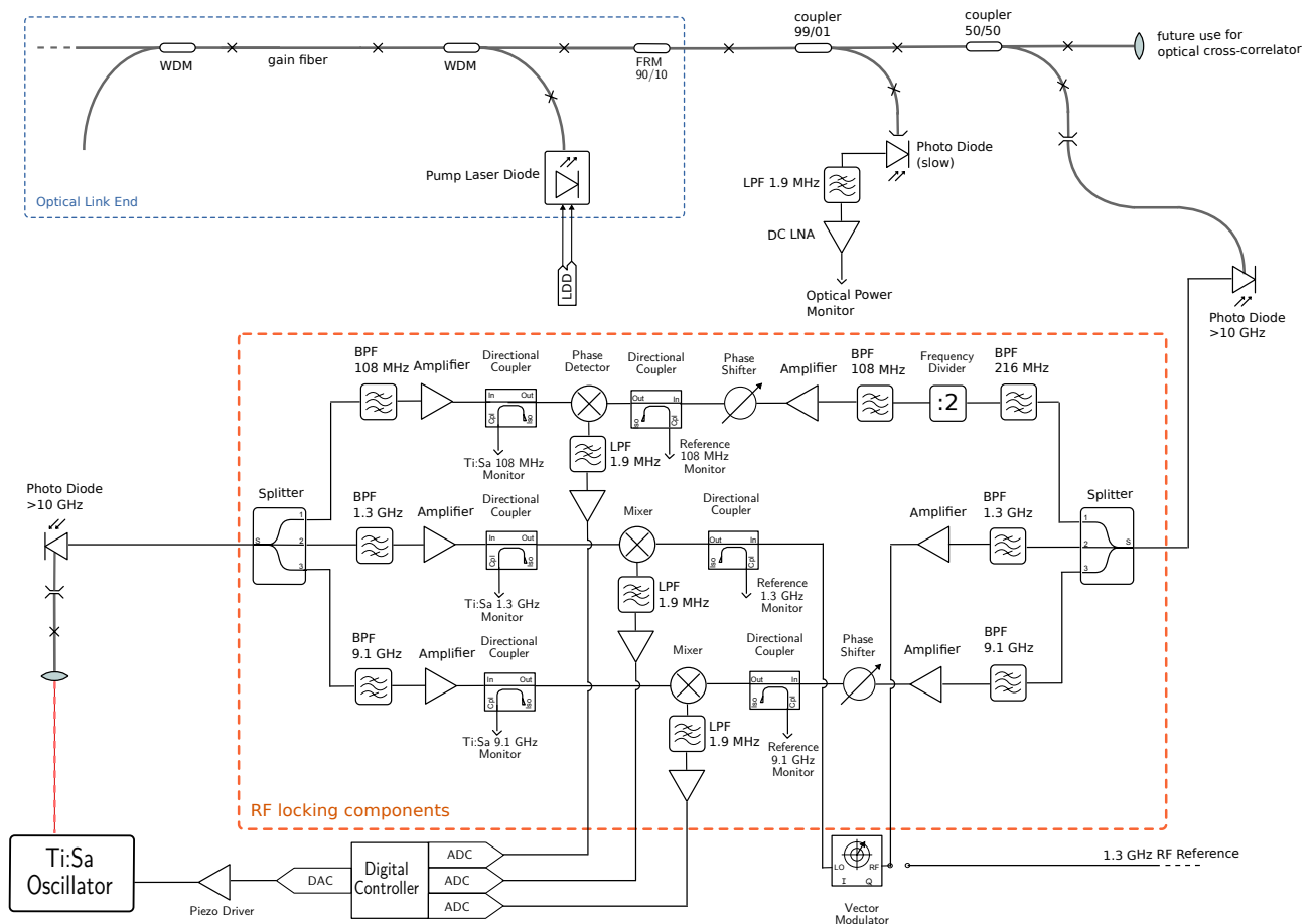
Figure 2: Block diagram of the main components for an RF-based lock of a 108 MHz Ti:Sapphire laser oscillator to the optical synchronization system of FLASH.
