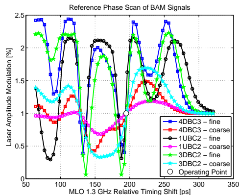
Figure 5: Simultaneous signal scan with three BAMs around the reference 1.3 GHz phase of the MLO at 92 deg or 197 ps.
