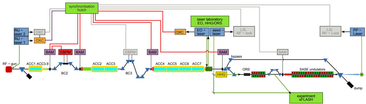
Figure 1: Schematic of the laser-based synchronisation system at the upgraded FLASH accelerator facility.
