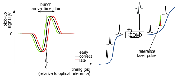
Figure 2: Schematic of the BAM detection scheme utilising electro-optical modulation.
