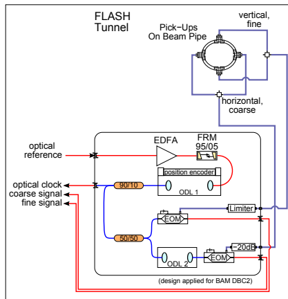
Figure 3: Schematic of the latest optical front-end design of the most recent BAM, installed after the first bunch compressor.
