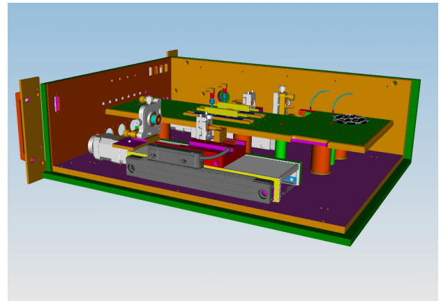
Figure 4: Schematic of the most recent BAM chassis. Visible are the two motorised delay stages and the four posts for the peltier elements underneath the aluminium plate on which both EOMs are installed.
