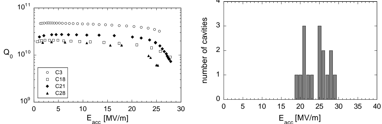
FIG. 14. (a) Excitation curves of the best 9-cell resonator of each of the four manufacturers. (b) Distribution of maximum gradients for the resonators of class 1, requiring a quality factor Q_0 \geq 5 \times 10^9 .
